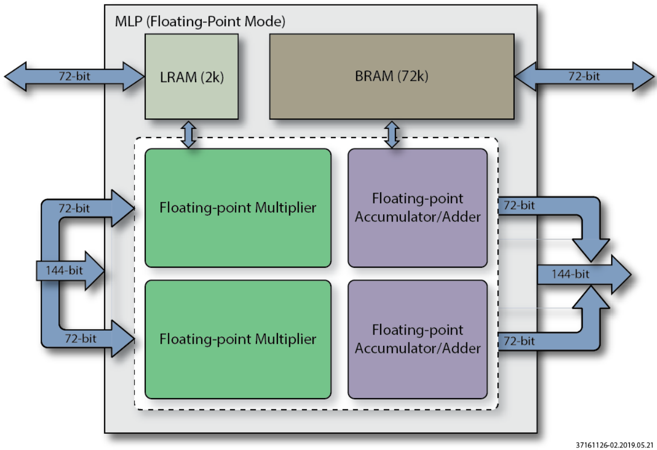
Figure 2: MLP Using Floating-Point Mode
